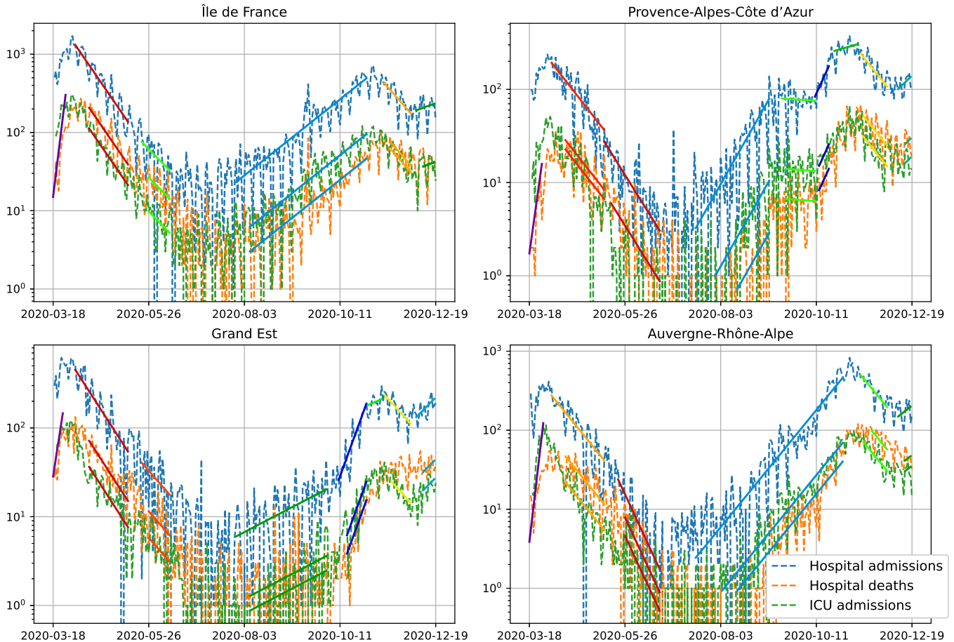
Figure 3: Growth rates of the cumulative number of infected individuals before, during and after lockdown in France, deduced from the number of hospital admissions, ICU admissions and hospital deaths in each patch. In each instance, an exponential curve was fitted simultaneously to each cumulative number of hospital admissions, ICU admissions and deaths.
