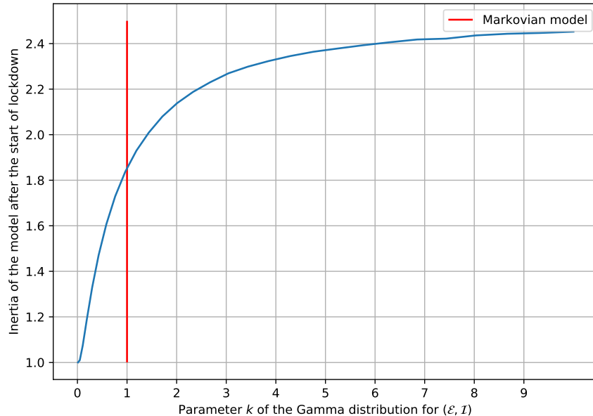
Figure S1: Inertia of the model of Definition 1 around a change in the contact rate, measured by the ratio (20). For each value of k , we consider that \mathcal{E} and \mathcal{I} are independent Gamma random variables with parameters (k, m_E/k) and (k, m_I/k) , respectively, with m_E = 2 and m_I = 5 . The Markovian ODE model corresponds to k = 1 (red vertical line). We can see that, for this choice of distributions, decreasing the variance of (\mathcal{E}, \mathcal{I}) increases the inertia of the model with memory.
