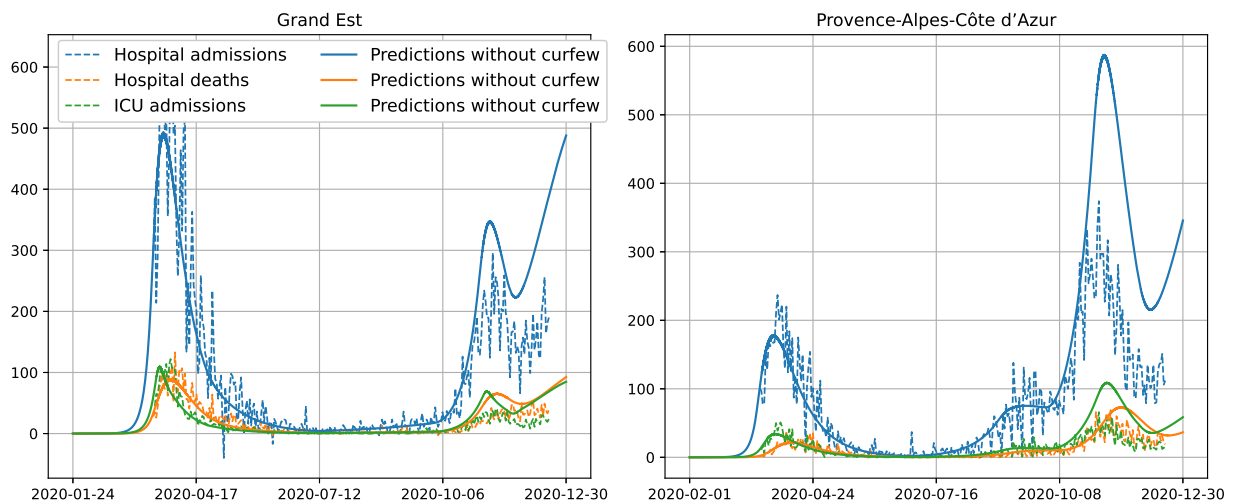
Figure S2: Model predictions of hospital admissions, ICU admissions and hospital deaths in the Grand Est and PACA regions without accounting for the (putative) effect of curfew before the second lockdown. To compute this, we assumed a single change of contact rate on October 30, with the rate computed from the halving time during the second lockdown.
