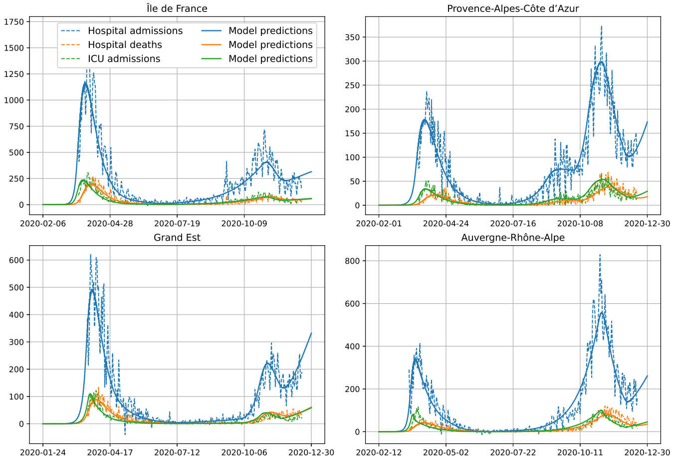
Figure 5: Model predictions and hospital data throughout the epidemic in four regions. In each region, we confront the daily hospital admissions, ICU admissions and hospital deaths due to Covid-19 to the predictions of our model. The model starts with a single infected individual at a different date in each region, and ends on December 31. The value used for the infection fatality ratio f was 0.5%, following [25], and the proportion of reported individuals was 0.8.
