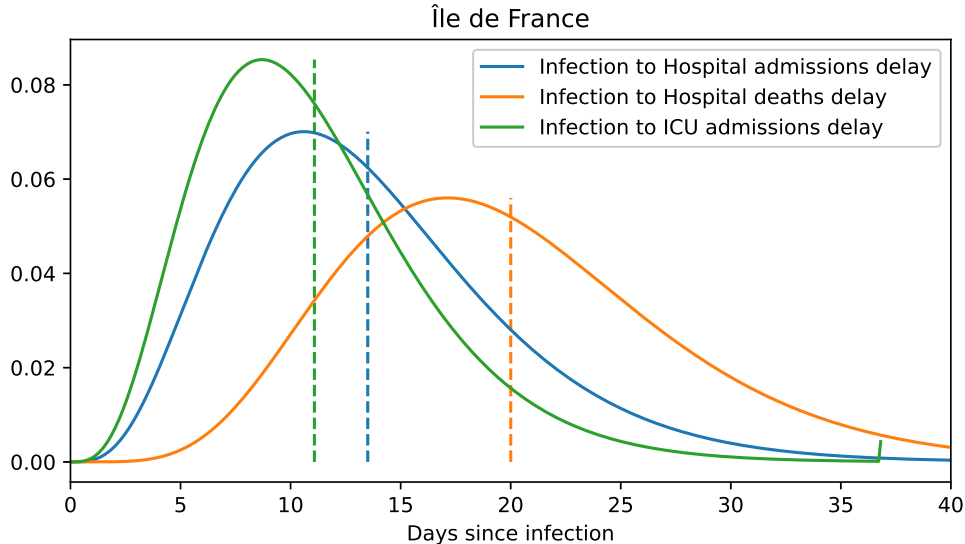
Figure 4: Probability density functions of the delays between infection and hospital admission (blue), ICU admission (green) and Hospital death (orange) estimated in Île-de-France. Means are indicated in dashed vertical lines.
