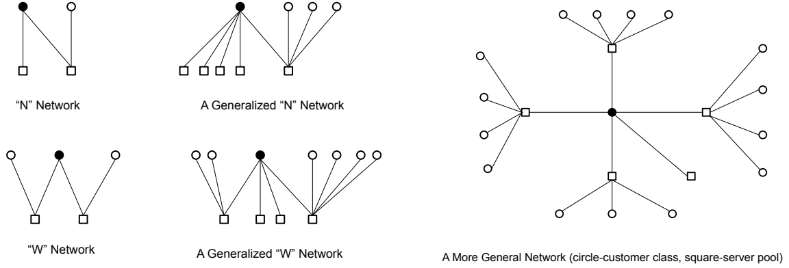
Figure 1. Examples of networks with a single dominant class
