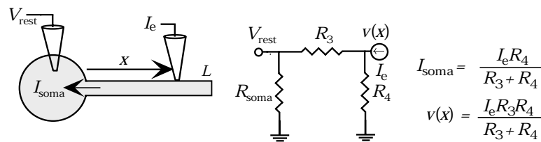
Figure 6.12 The Rall model with static current injected a distance x along the equivalent cable while the soma is clamped at its resting potential. The schematic at left shows the recording set up. The potential at the site of the current injection and the current entering the soma are measured. The central diagram is the equivalent circuit for this case, and the corresponding formulas for the somatic current and dendritic voltage are given at the right. R_{\text{soma}} is the membrane resistance of the soma, and R_3 and R_4 are the resistances given in equations 6.26 and 6.27.
