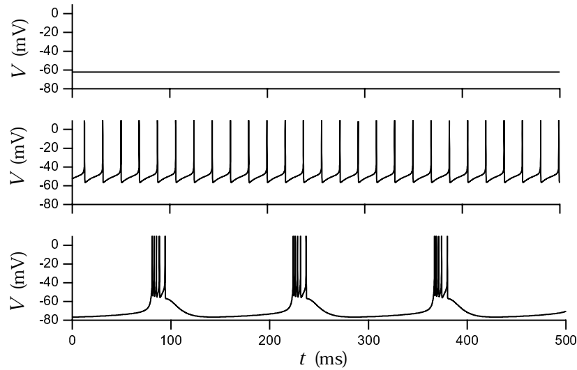
Figure 6.3 Three activity modes of a model thalamic neuron. Upper panel: with no electrode current the model is silent. Middle panel: when a positive current is injected into the model neuron, it fires action potentials in a regular periodic pattern. Lower panel: when negative current is injected into the model neuron, it fires action potentials in periodic bursts. (Adapted from Wang, 1994)
