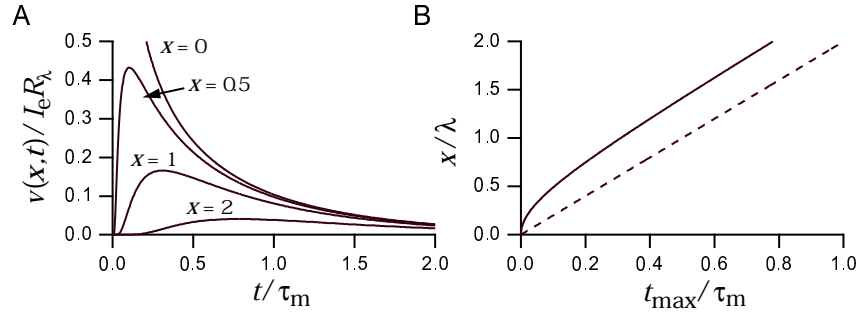
Figure 6.8 Time-dependence of the potential on an infinite cable in response to a pulse of current injected at the point x = 0 at time t = 0 . A) The potential is always largest at the site of current injection. At any fixed point, it reaches its maximum value as a function of time later for measurement sites located further away from the current source. B) Movement of the temporal maximum of the potential. The solid line shows the relationship between the measurement location x , and the time t_{\max} when the potential reaches its maximum value at that location. The dashed line corresponds to a constant velocity 2\lambda/\tau_m .
