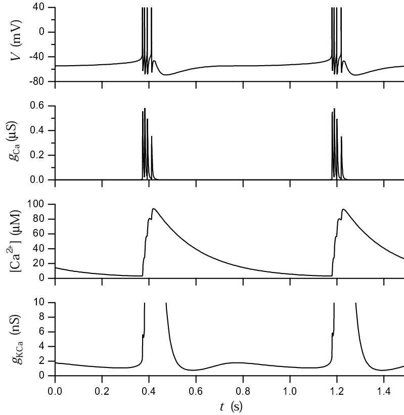
Figure 6.4 Periodic bursting in a model of a crustacean stomatogastric ganglion neuron. From the top, the panels show the membrane potential, the \text{Ca}^{2+} conductance, the intracellular \text{Ca}^{2+} concentration, and the \text{Ca}^{2+} -dependent \text{K}^+ conductance. The \text{Ca}^{2+} -dependent \text{K}^+ conductance is shown at an expanded scale so the reduction of the conductance due to the falling intracellular \text{Ca}^{2+} concentration during the interburst intervals can be seen. In this example, \tau_{\text{Ca}} = 200 ms. (Simulation by M. Goldman based on a variant of a model of Turrigiano et al., 1995 due to Z. Liu and M. Goldman.)
